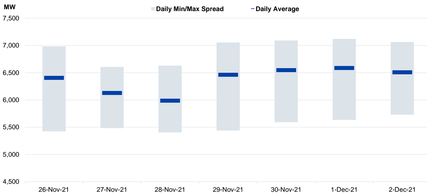
Figure 6: Seven Days Forecasted Demand Average-Max-Min
