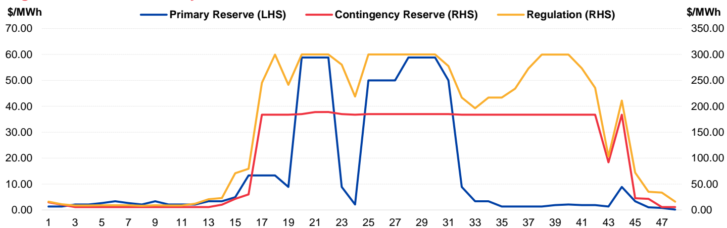
Figure 2: Periodic Ancillary Prices
