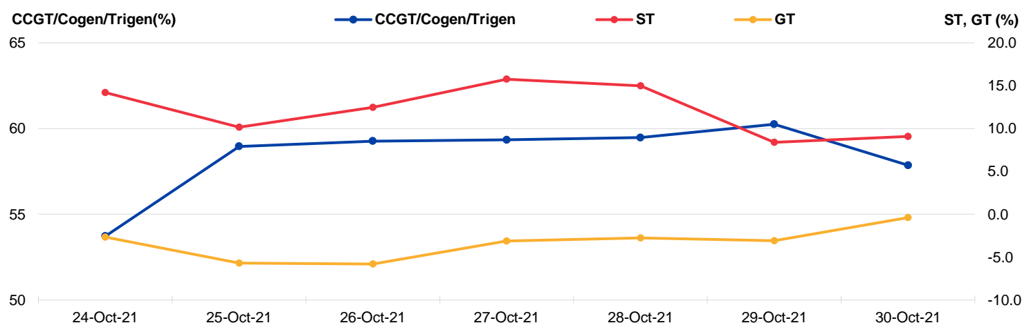
Figure 7: Daily Generation Plant Utilization Rate
