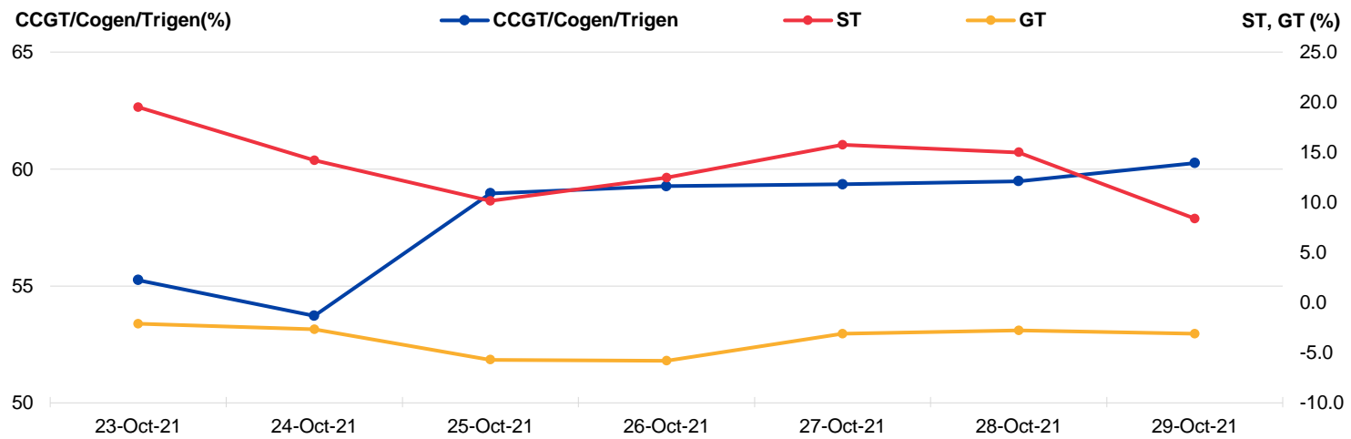
Figure 7: Daily Generation Plant Utilization Rate
