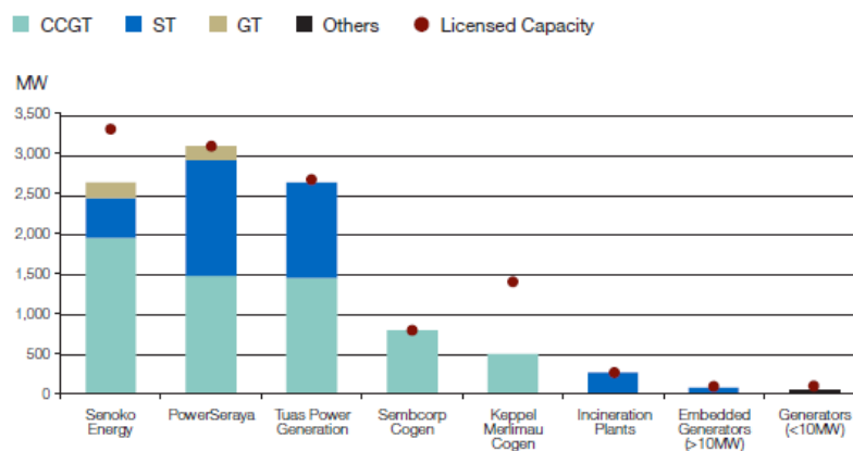
Figure 1: Generation Capacity 2010: Registered Versus Licensed
